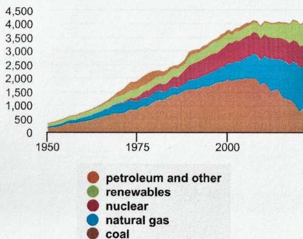
U.S. electricity generation by major energy source, 1950-2021
